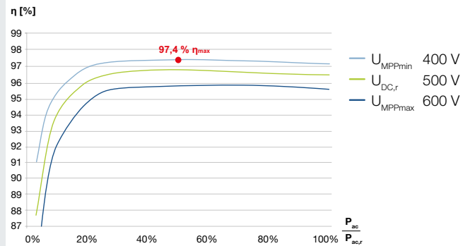
PIKO MP plus 3.0 to 4.6 with 2 MPP Tracker
